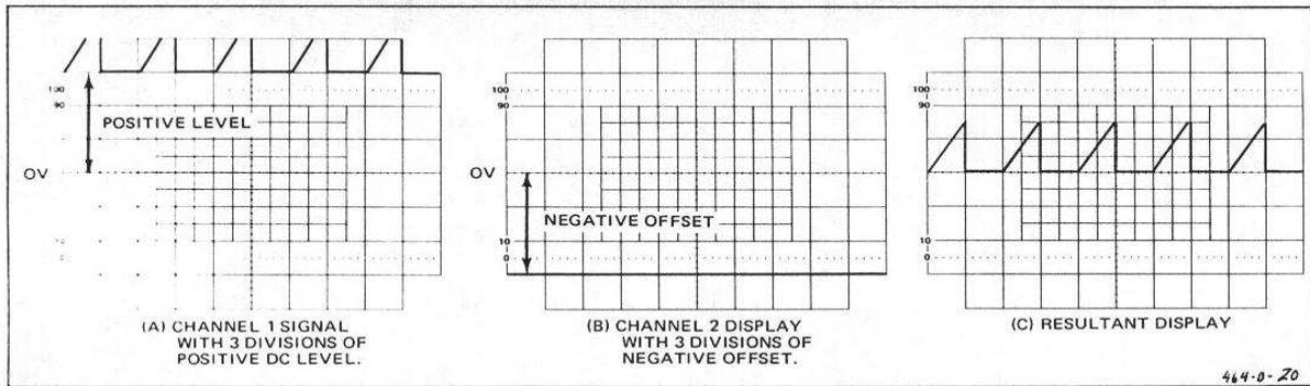
Fig. 15. Algebraic addition.
