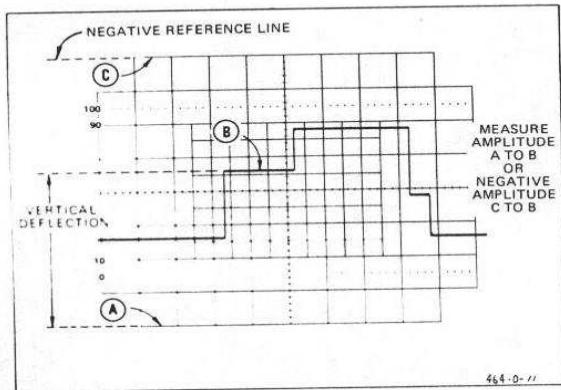
Fig. 6. DC voltage with respect to a reference line.
