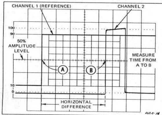
Fig. 9. Time differences between two pulses.
