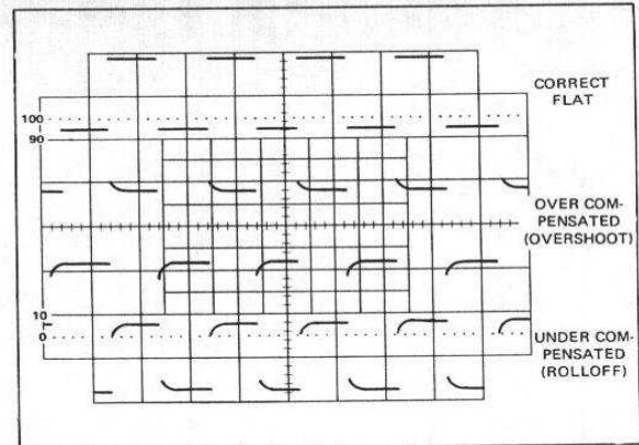
Fig. 4. Probe compensation.
