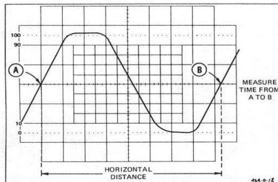
Fig. 7. Time duration between points on a waveform.
