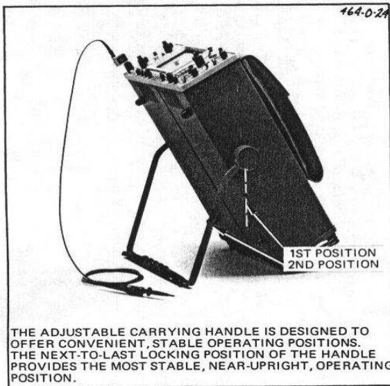
Fig. 3. Tilted operation.
