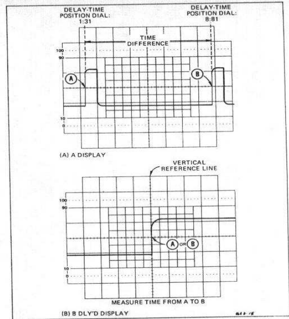
Fig. 13. Time difference using delaying sweep.
