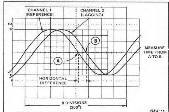
Fig. 10. Phase difference.
