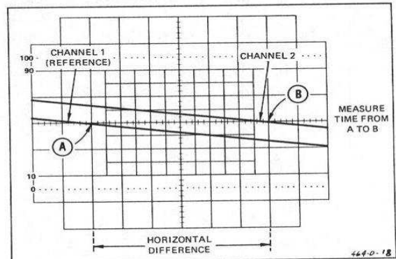
Fig. 11. High-resolution phase difference with increased sweep rate.
