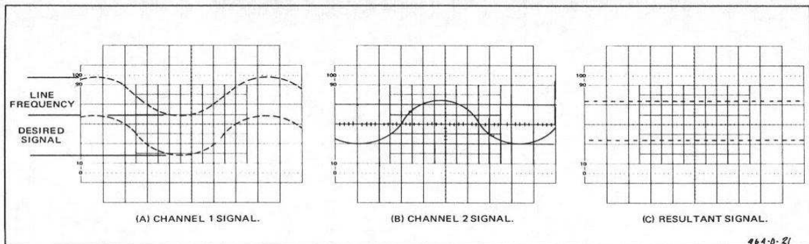
Fig. 16. Common mode rejection.
