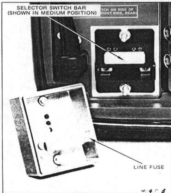
Fig. 1. Regulating range selector and line fuse.
