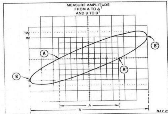
Fig. 12. Phase difference from an X-Y display.
